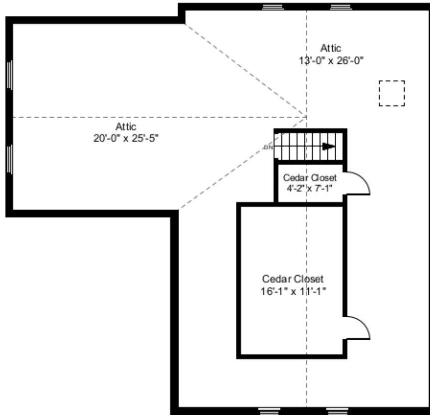
Attic Plan Ceiling Height = 9'-10"
