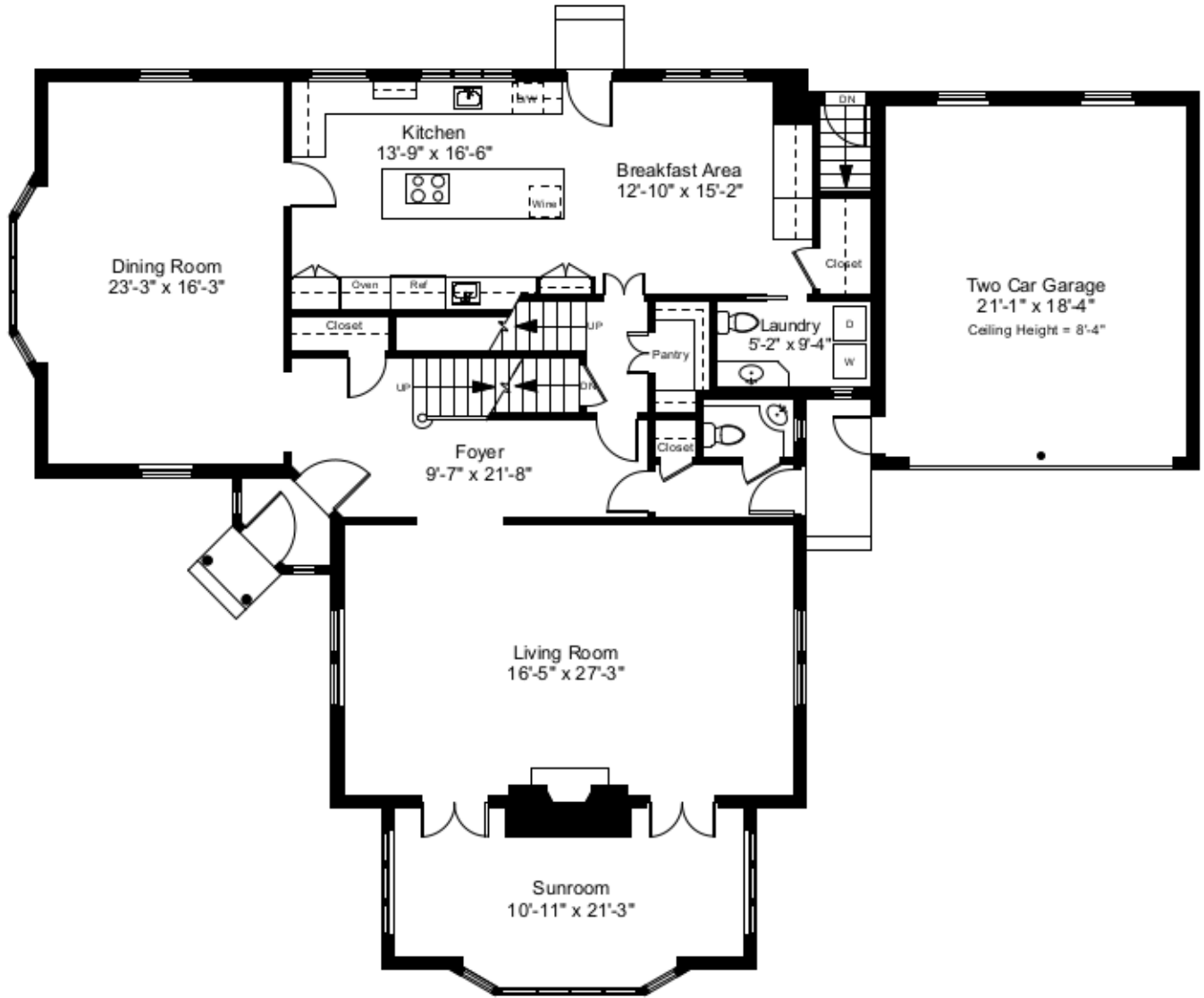
First Floor Plan Ceiling Height = 8'-8"
